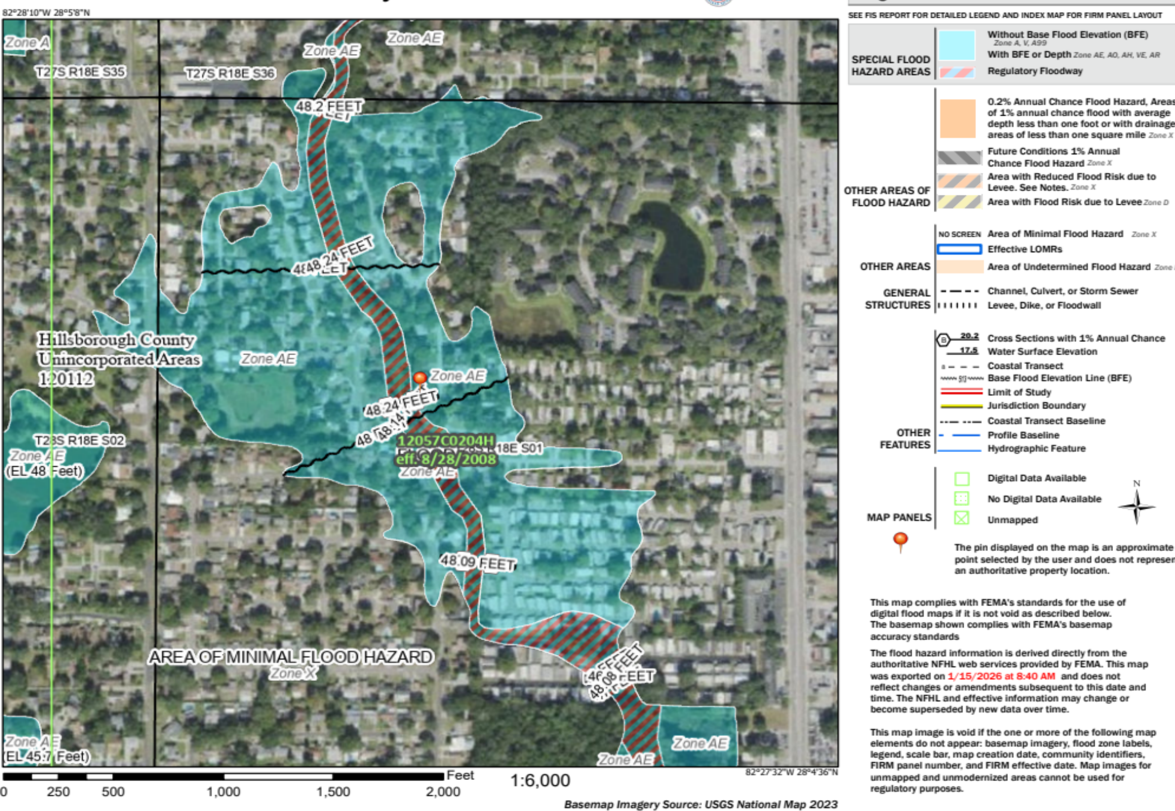
National Flood Hazard Layer FIRMette
