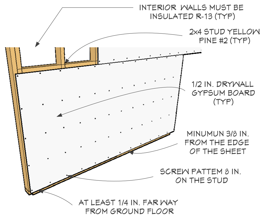
INTERIOR WALL DETAIL (TYP.)
